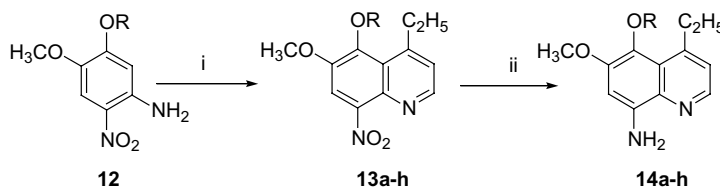
Scheme 4. Reagents and conditions: (i) 1-chloro-3-pentanone, 85% o - \text{H}_3\text{PO}_4 , \text{As}_2\text{O}_3 , 80 °C, 3 h; (ii) raney-Ni/ \text{H}_2 , EtOH, 45 psi, rt.
