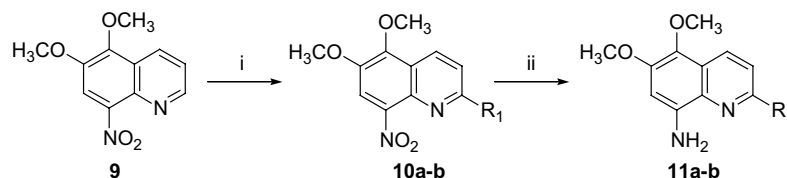
Scheme 3. Reagents and conditions: (i) R_1\text{CO}_2\text{H} , \text{AgNO}_3 , (\text{NH}_4)_2\text{S}_2\text{O}_8 , 10% \text{H}_2\text{SO}_4 , \text{CH}_3\text{CN} , 70–80 °C; (ii) raney-Ni/ \text{H}_2 , EtOH, 45 psi, rt.
