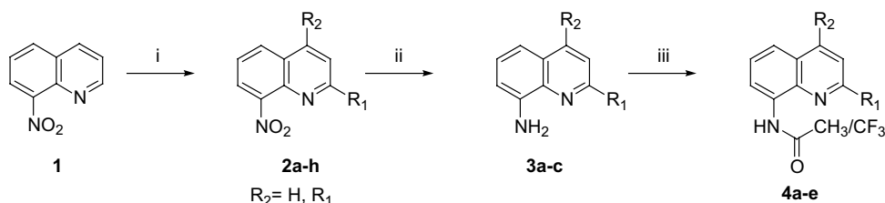
Scheme 1. Reagents and conditions: (i) R_1CO_2H , AgNO_3 , (NH_4)_2S_2O_8 , 10% H_2SO_4 , CH_3CN , 70–80 °C; (ii) raney-Ni/ H_2 , EtOH, 45 psi, rt; (iii) (CH_3CO)_2O/C_5H_5N or (CF_3CO)_2O , rt.
