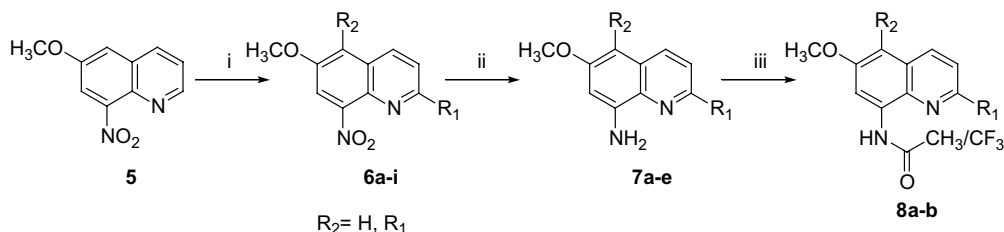
Scheme 2. Reagents and conditions: (i) R_1\text{CO}_2\text{H} , \text{AgNO}_3 , (\text{NH}_4)_2\text{S}_2\text{O}_8 , 10% \text{H}_2\text{SO}_4 , \text{CH}_3\text{CN} , 70–80 °C; (ii) raney-Ni/ \text{H}_2 , EtOH, 45 psi, rt; (iii) (\text{CH}_3\text{CO})_2\text{O}/\text{C}_5\text{H}_5\text{N} or (\text{CF}_3\text{CO})_2\text{O} , rt.
